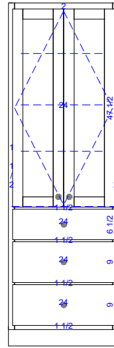
LDS-823-27 27"W x 84"H x 24"D
