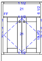
VDS-SB820-24 24"W x 34½"H x 21"D
