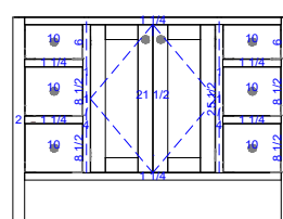
VCA-321S-48 48"W x 35"H x 21½"D
