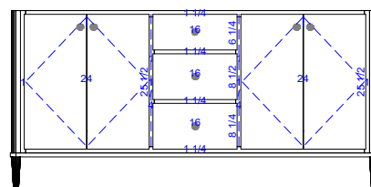
VCW-251D-72 72"W x 35"H x 21½"D
