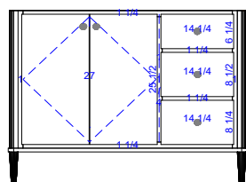
VCW-251-48-L OR VCS-251-48-R 42"W x 35"H x 21½"D
