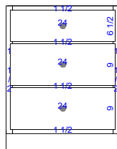
VDS-B821-27 27"W x 34½"H x 21"D
