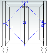
VOC-560-30 30"W x 35"H x 21 1/2"D
