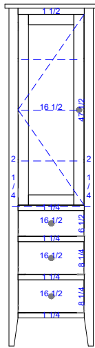
LCS-433-21-L OR LCS-433-21-R 21"W x 84"H x 24"D
