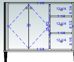
VCW-251-42-L OR VCS-251-42-R 42"W x 35"H x 21½"D
