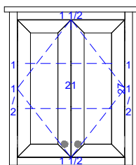
WOC-565-24 24"W x 30"H x 10"D
